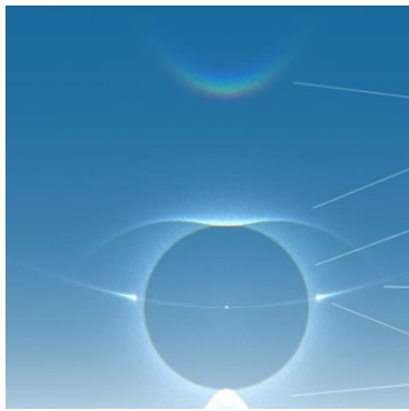
NORMAL PARHELIA
