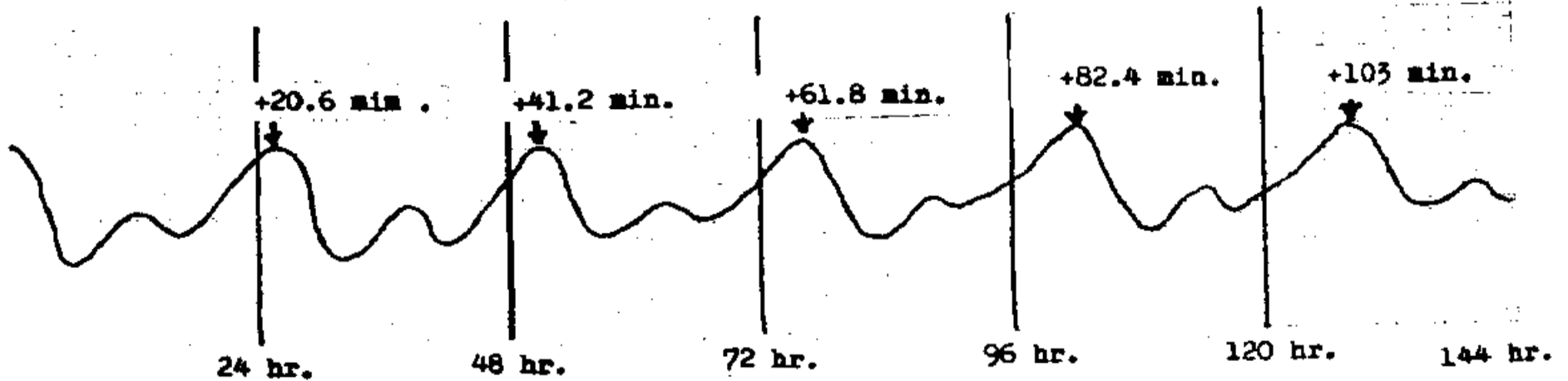
FIG. 30. IDEALIZED REPRESENTATION OF THE "FREE-RUNNING" CYCLE OF ACTIVITY OF A PLANT OR ANIMAL (ORGANISM) LEFT IN CONTINUOUS DARKNESS. IN THE ABSENCE OF THE LIGHT "TRIGGER" OF THE SUN, THE PLANT OR ORGANISM WILL TAKE UP A RHYTHM UNIQUELY ITS OWN. WE SUGGEST THAT THE PERIOD THAT IS A MEAN BETWEEN ALL THE EXTREMES FOR ALL PLANTS AND ANIMALS WILL APPROXIMATE TO THE COSMIC DAY OF 24 HOURS, 20 MINUTES AND 36 SECONDS. THE BIOLOGIST HAS BEEN CAUSED TO ADOPT THE TERM "CIRCADIAN" MEANING "ROUND ABOUT A DAY" BECAUSE OF AN IGNORANCE OF THE REAL AND CONSTANT BASE OF THE TIME UNIT. THE BIOLOGICAL AND OTHER PHYSICAL RHYTHMS DO VARY IN RESPONSE TO THE LUNAR POSITION AND ITS CORRELATE WITH THE SOLAR POSITION. BUT UNDERNEATH THE PHENOMENAL MANIFESTATION OF RHYTHMS WHICH PRECESS AND RETARD IN PERIODICITY, THERE SHALL BE FOUND THE COSMIC BASE OF 24 HOURS, 20 MINUTES AND 36 SECONDS.
